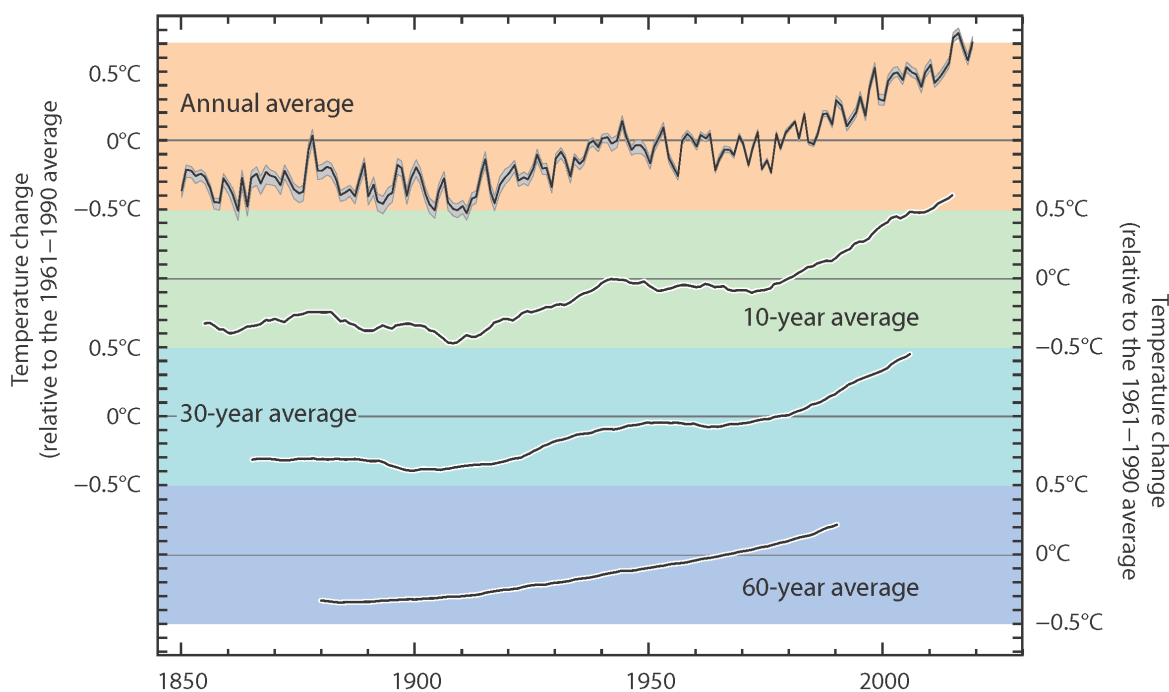
Figure 3. The average global surface temperature is about 2.0 degrees Fahrenheit (1.2 degrees Celsius) warmer than in the two decades before 1900. Averages taken over 10-year, 30-year, and 60-year intervals smooth out the interannual variability and more clearly reveal the trend of constantly increasing temperatures. Source: NAT'L ACAD. OF SCI. & THE ROYAL SOC'Y, CLIMATE CHANGE: EVIDENCE & CAUSES UPDATE 2020, at 11 (2020).
